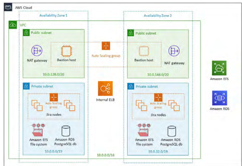
Architecture Diagram
